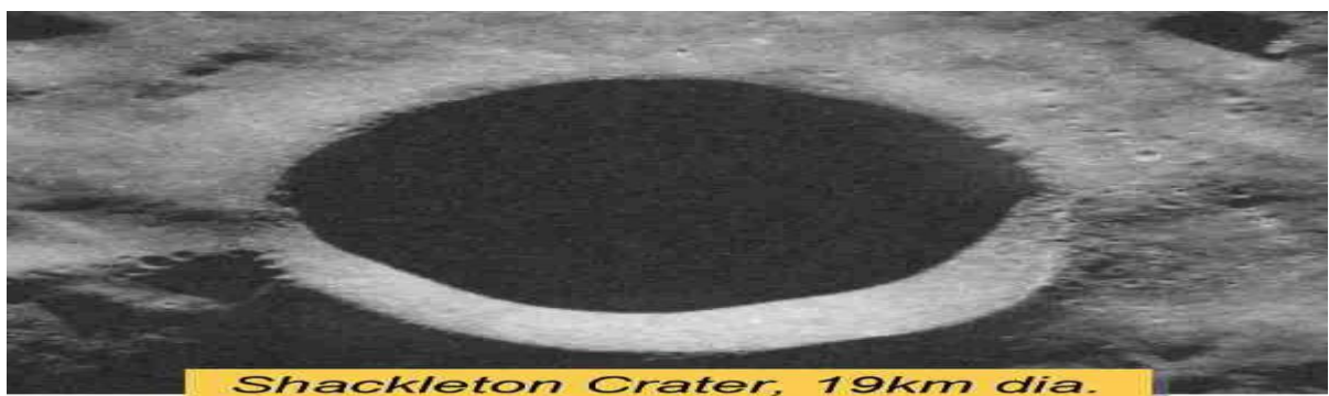
Shackleton Crater, 19km dia. (lunar South Pole) 2005 Arecibo radar image
