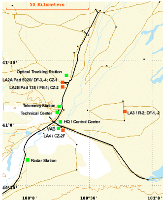
Shenzhou-5
