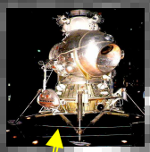
Soyuz 7K-LOK/Luna 24
