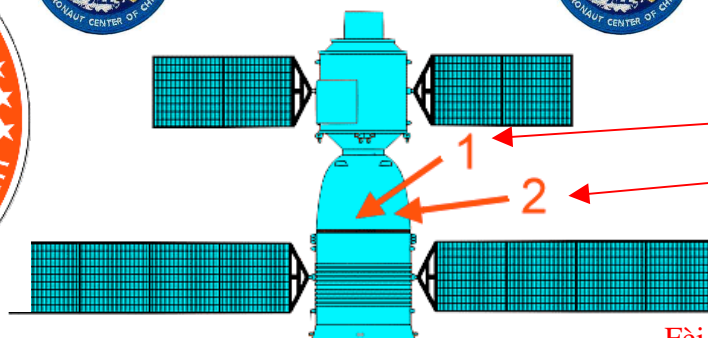
Shenzhou-6
