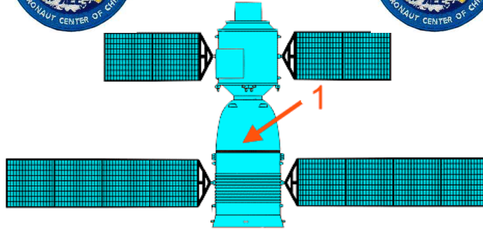
Shenzhou-8
