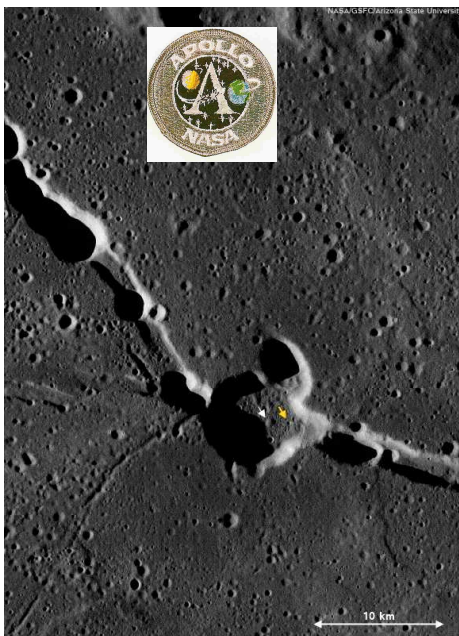
Apollo 19
