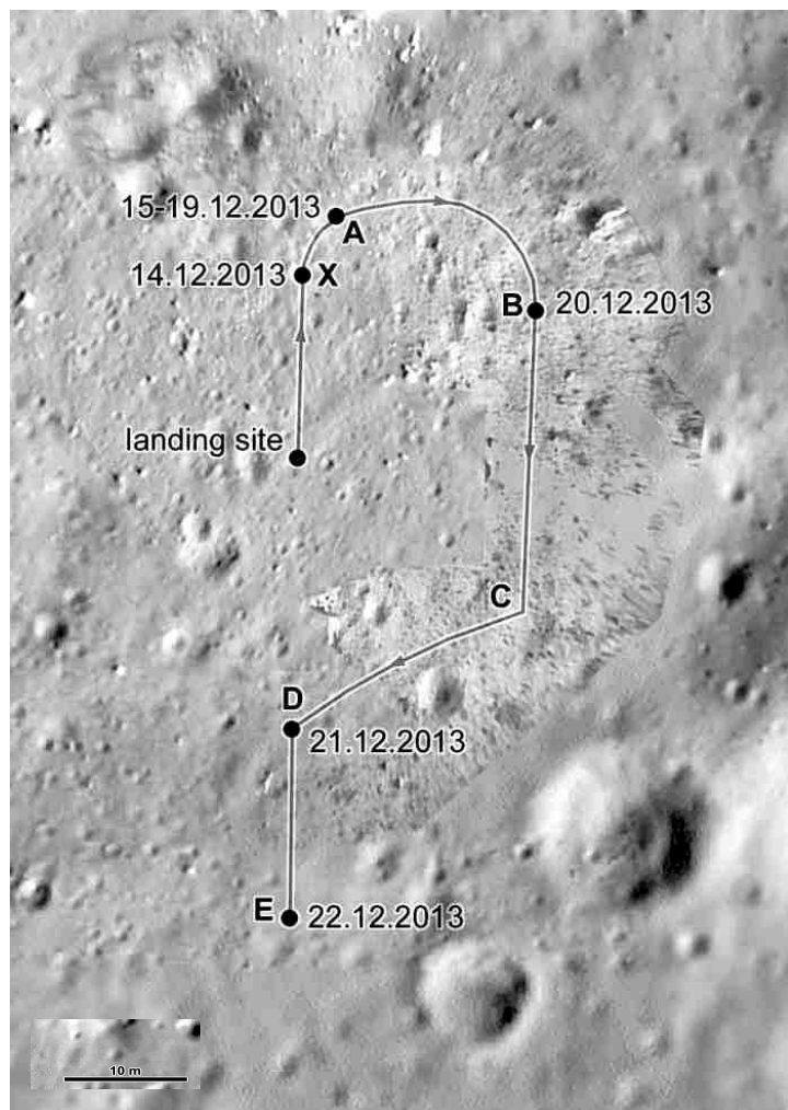
The map shows the Jade Rabbit's journey during the first week after touch-down.
