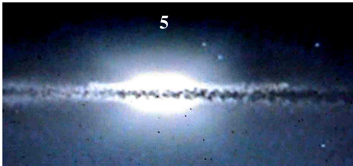
The Milky Way seen from the side, the nucleus is described as being similar to a peanut. A result of efforts made by, among others, Galilei, Newton, Einstein and NASA concerning our galaxy.
