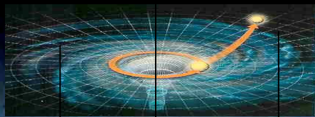
The road into the interior of our galaxy, the Milky Way
