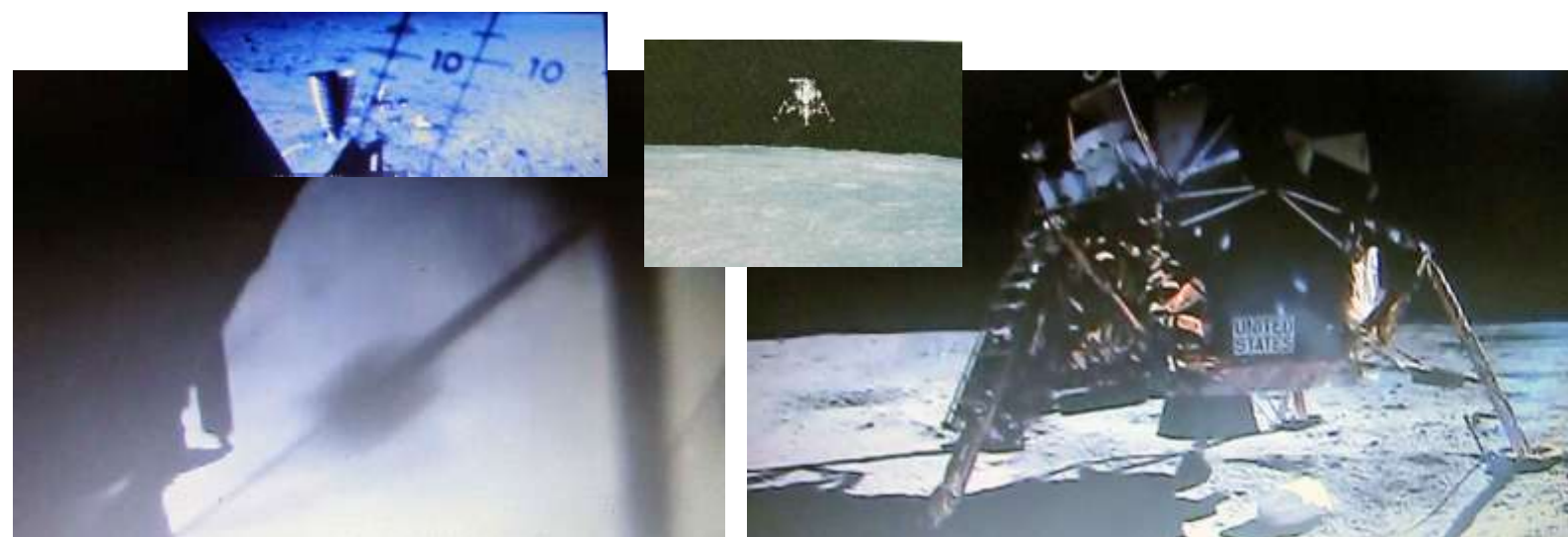
On 19 November 1969 Intrepid landed on the Moon, at Ocean of Storms. Picture: lunar module Intrepid, astronauts Conrad and Bean.
