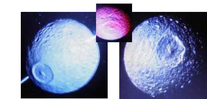
Mimas, spherical object which vibrates around Saturn.
