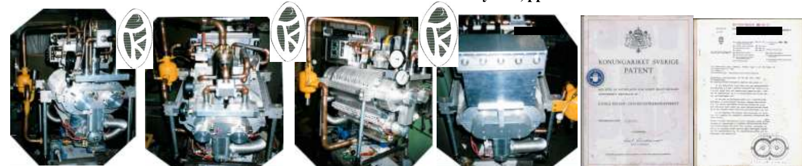
Tibor Kemény. Expansions Turbin Motor, prototyp – 1982. Patent in Sverige 1984,
