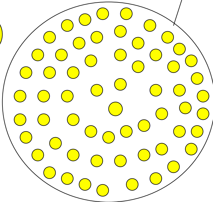
This is the new model of an atom which has no neutrons or electrons, i.e. no binary star system. Note that this is my own theory.
