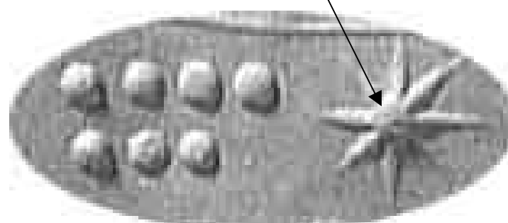
Our solar system, II, according to Sumerian astronomy. It has seven planets. At the centre is the neutron sun, a star. This picture is from the time of An.
