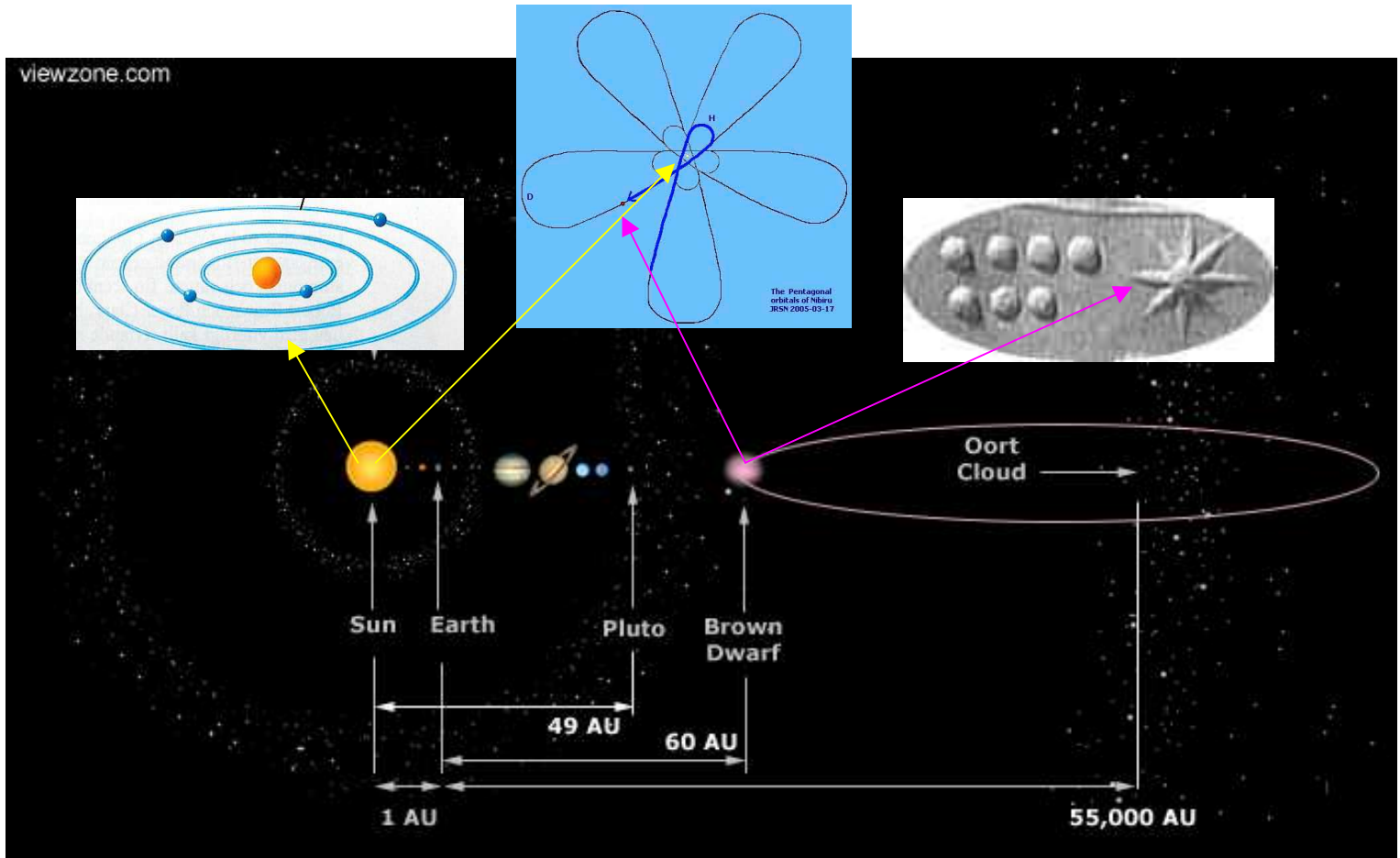
Above is our solar system with binary stars. The neutron star Nemesis has a pentagon orbit around the Sun, around 3,800 years. The Earth and the Moon, our nearest celestial body, exist in this binary star system.
